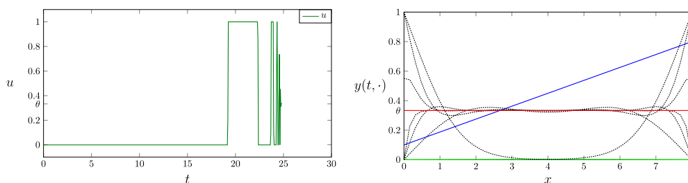
Figure 9. Optimal control u and resulting state y(t, \cdot) from time 0 (in blue), to t_f (in red) with intermediate times 0.7t_f (in green), and several others from 0.95t_f to t_f (in dashed line).
