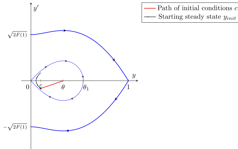
Figure 3. The path c of initial conditions, from those of y_{\text{init}} (black dot) and those for \theta . The state y_{\text{init}} is also depicted.
